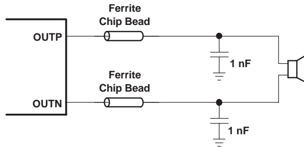
Figure 34. Typical Ferrite Chip Bead Filter (Chip bead example: Fair-Rite 2512067007Y3)
